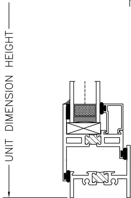
3 CASEMENT @ SILL
