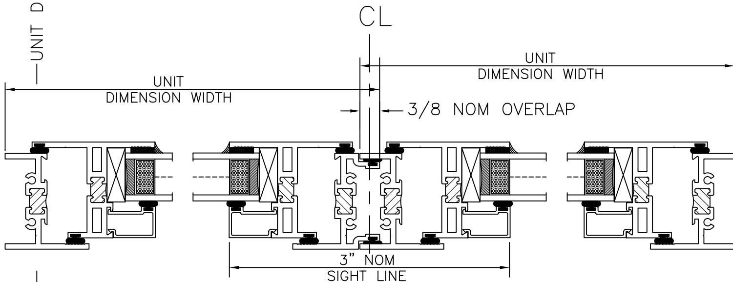
2 CASEMENT @ JAMB
