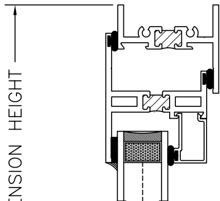
1 CASEMENT @ HEAD
