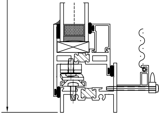
3 CASEMENT @ SILL
