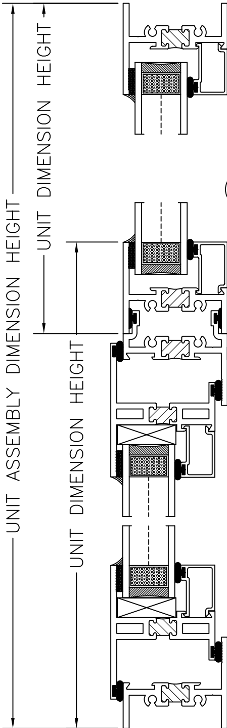
10 FIXED OVER PROJECT OUT @ SILL
