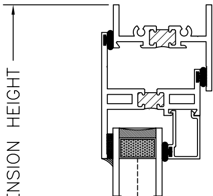
1 CASEMENT @ HEAD
