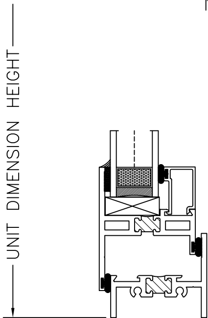
3 CASEMENT @ SILL
