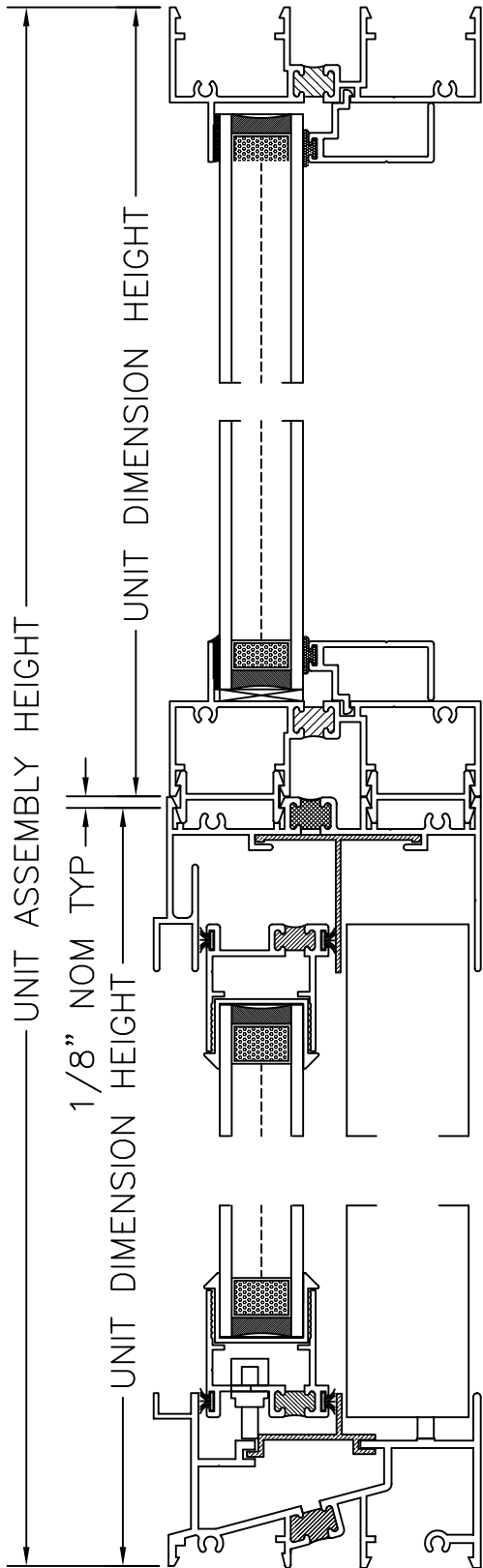
1 FIXED OVER SLIDER WINDOW @ VERTICAL SECTION
