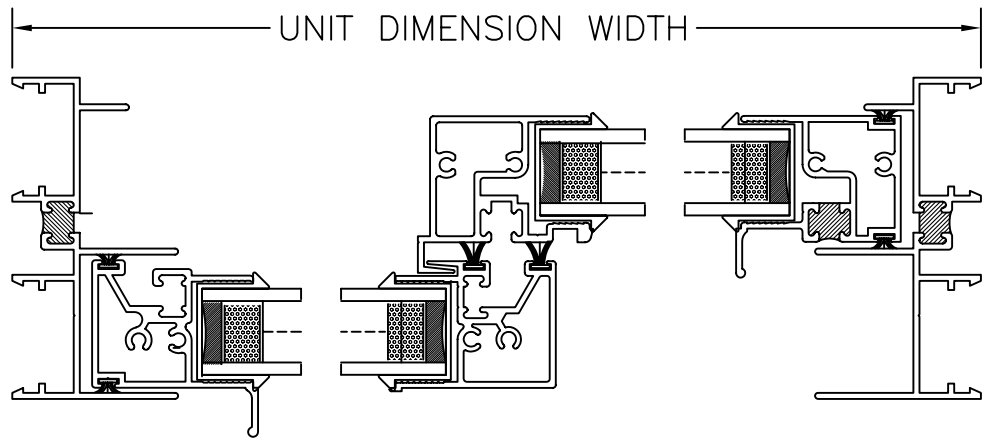
2 FIXED OVER SLIDER WINDOW @ HORIZONTAL SECTION
